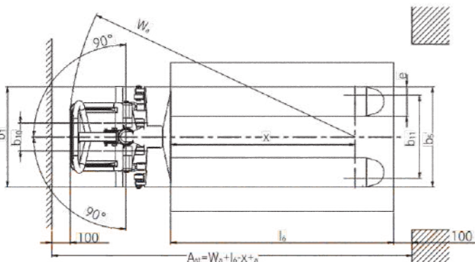
HPT 10 XE top view
