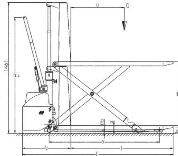
HPT 10 XE side view
