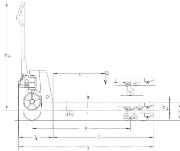
HPS 20 side view
